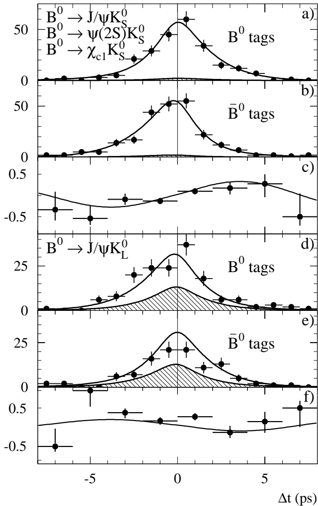
FIG. 2: Number of \eta_f = -1 candidates ( J/\psi K_S^0 , \psi(2S)K_S^0 , and \chi_{c1}K_S^0 ) in the signal region a) with a B^0 tag N_{B^0} and b) with a \bar{B}^0 tag N_{\bar{B}^0} , and c) the asymmetry (N_{B^0} - N_{\bar{B}^0})/(N_{B^0} + N_{\bar{B}^0}) , as functions of \Delta t . The solid curves represent the result of the combined fit to all selected CP events; the shaded regions represent the background contributions. Figures d)–f) contain the corresponding information for the \eta_f = +1 mode ( J/\psi K_L^0 ). The likelihood is normalized to the total number of B^0 and \bar{B}^0 tags. The value of \sin 2\beta is independent of the individual normalizations and therefore of the difference between the number of B^0 and \bar{B}^0 tags.
