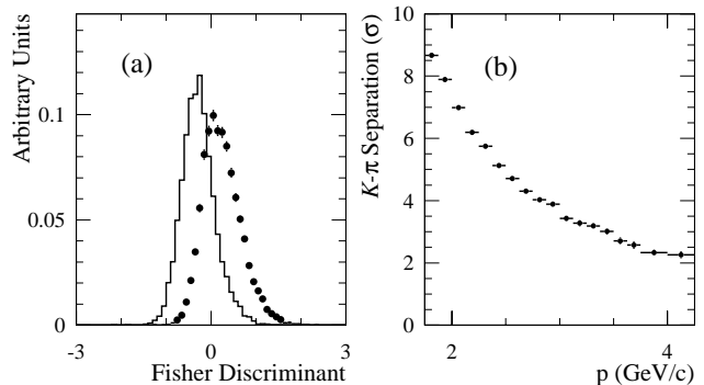
FIG. 1: (a) The distributions of the Fisher discriminant for Monte Carlo simulated B^0 \rightarrow h^+h'^- decays (histogram) and background events (points) in the m_{ES} sideband region 5.20 < m_{ES} < 5.27 \text{ GeV}/c^2 ; (b) the K - \pi separation, in units of standard deviations, as a function of momentum, derived from the Cherenkov angle measurements of kaon and pion tracks in a D^{*+} \rightarrow D^0\pi^+ control sample, as described in the text.
